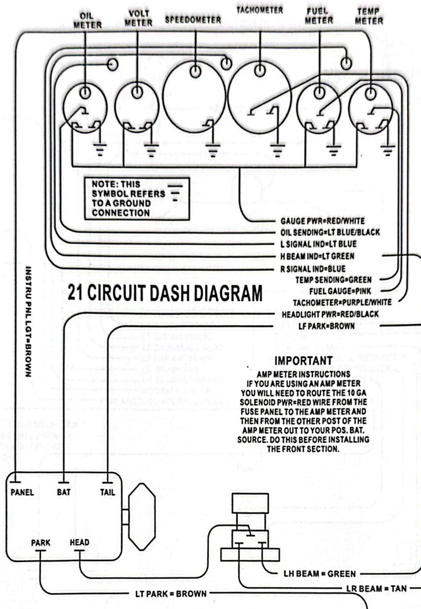
21 CIRCUIT FRONT SECTION DIAGRAM
