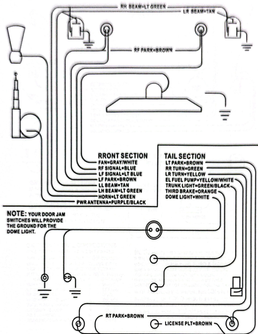
21 CIRCUIT TAIL SECTION DIAGRAM
